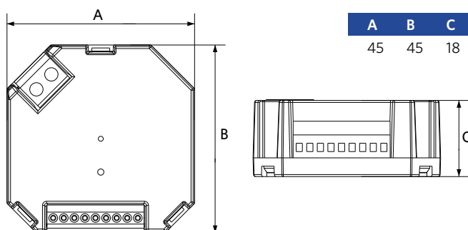
821017003400 - LEDSmart-BLE2-Multi-Switch-Module
